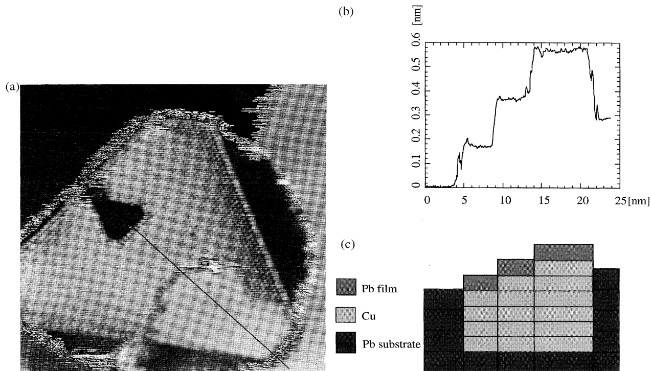
FIG. 3. (a) STM image of a type b Cu island. The lattice of the Pb overlayer as well as the Cu island lattice is rotated by 30^\circ with respect to the Pb substrate. The Pb overlayer exhibits the moiré pattern of Pb on Cu(111). As Fig. 2(a), this image has been slightly differentiated, and the height difference between various terraces has been reduced ( 20 \times 20 \text{ nm}^2 ). (b) Section through (a) marked by the line. (c) Model for the Cu island that best fits the section in (b). Each rectangle represents a single layer.
