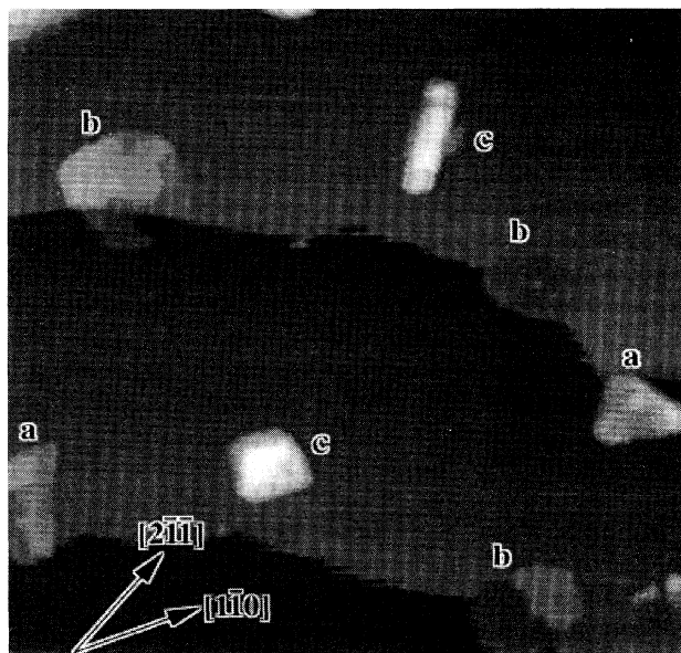
FIG. 1. STM image of Pb(111) after deposition of 0.94 ML Cu. Three different types of Cu islands are visible ( 100 \times 100 nm 2 ).
