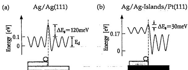
FIG. 3. Potential energy diagram characterizing the interlayer and intralayer diffusion in Ag homoepitaxy (a) and heteroepitaxy (b) at the (111) surfaces of Ag and Pt. The intralayer diffusion barriers are from Refs. [15] and [23], the difference in binding energy in case (b) from Ref. [22].
